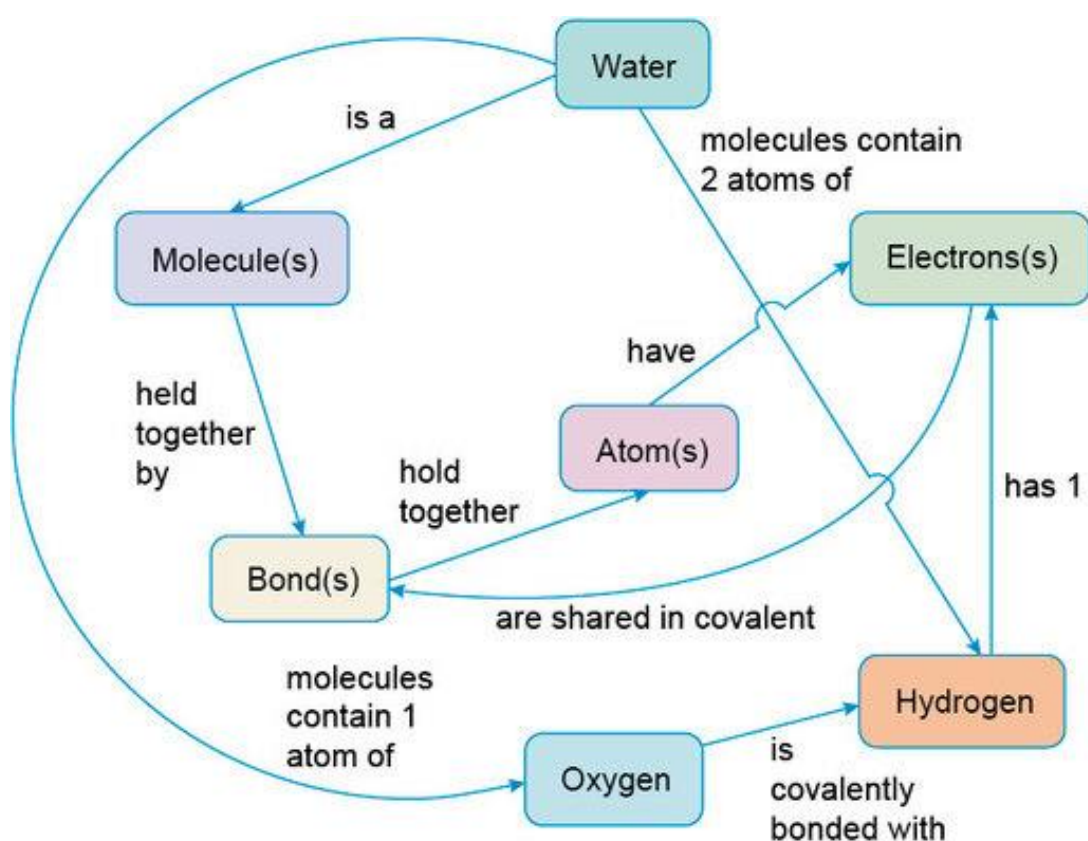
Figure 10 Adding details
