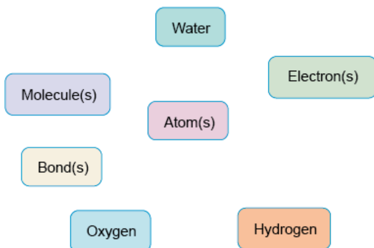
Figure 8 Arranging concepts
