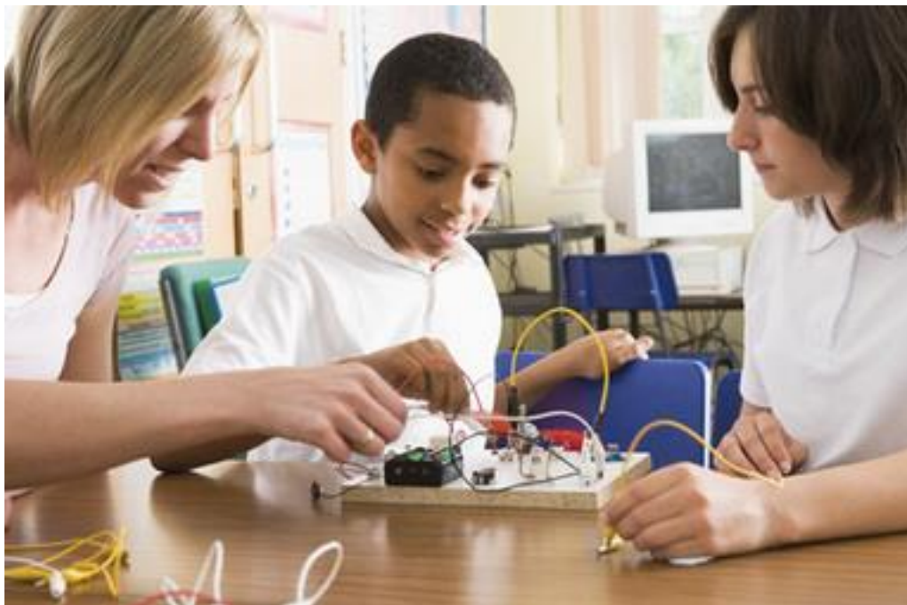
Figure 11 Making circuits
