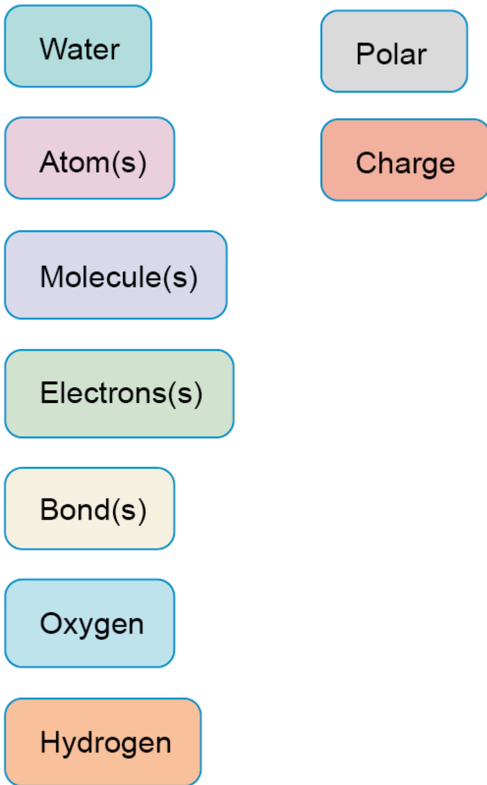
Figure 7 Sorting concepts
