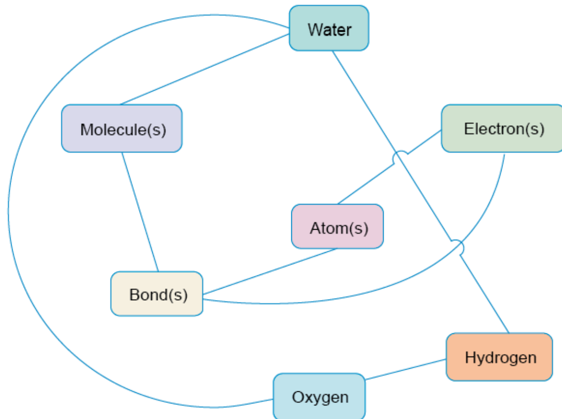
Figure 9 Linking concepts
