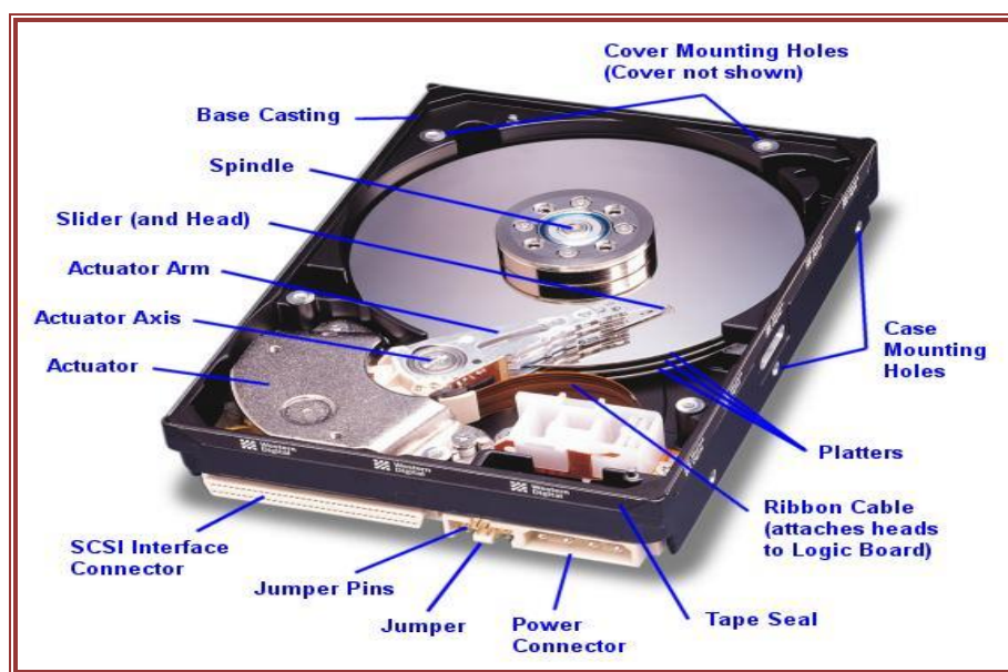
3.10-rasm. Mikrokompyuterdagi qattiq disk 6 .
