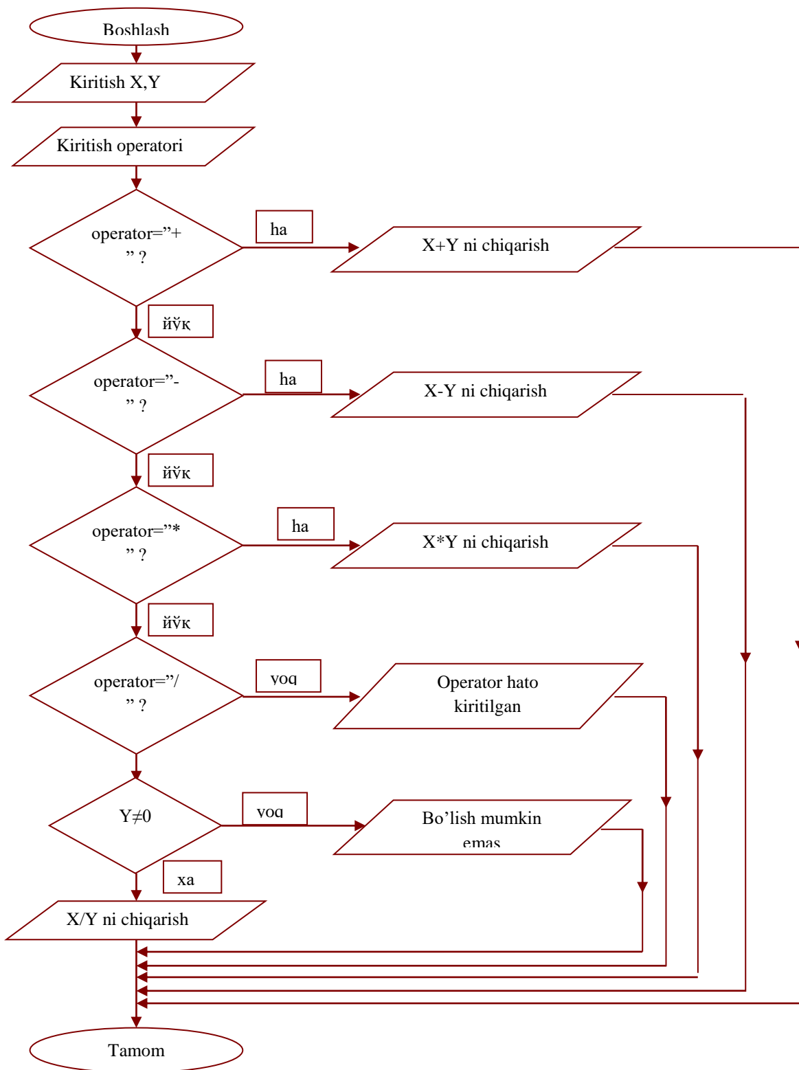
11.8-rasm. blok-chizmada sodda kalkulyatorning algoritmi 42
