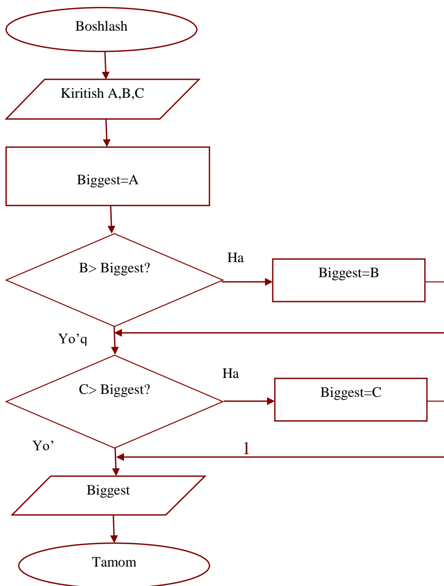
1.6-rasm. Uchta son ichidan eng kattasini topish
