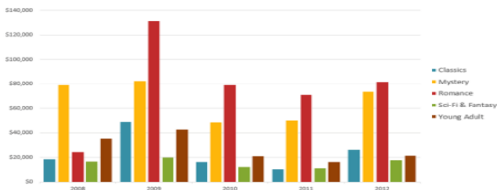
5.72-rasm. Gistogramma.
