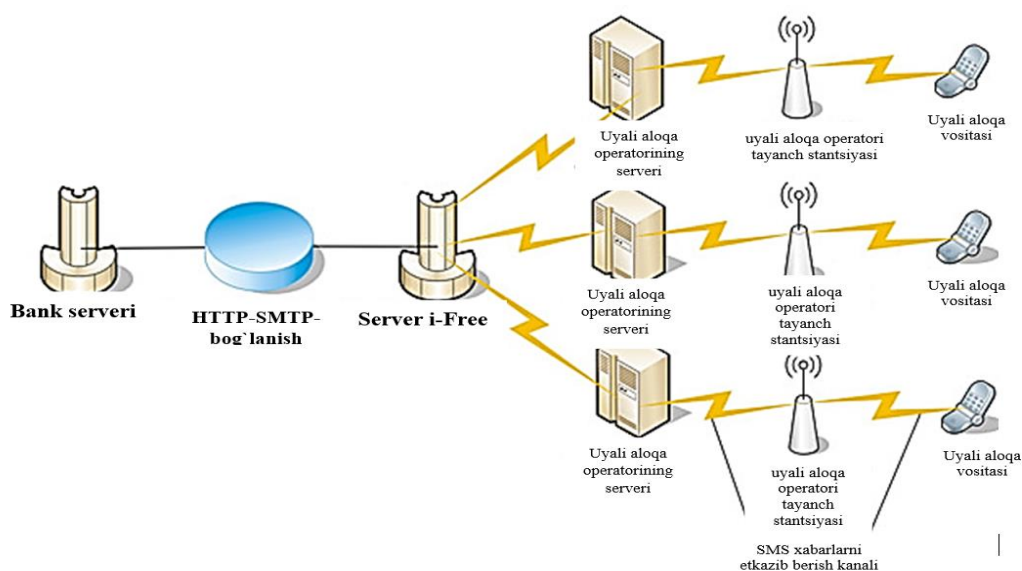
14.13-rasm. Bank serverining provayder serveriga ulanish sxemasi 159
